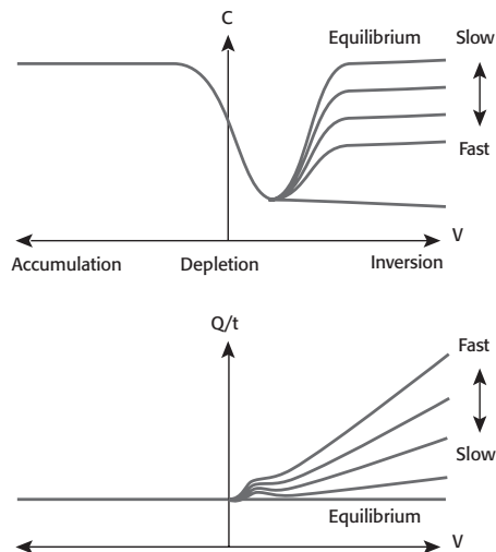
FIGURE 1: Model 595 C vs. V and Q/t vs. V Curves Q/t used to indicate the degree of equilibrium
