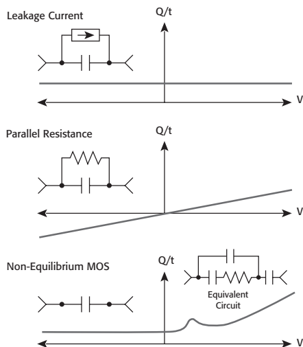
FIGURE 2: Q/t vs. V Curves used to diagnose leakage currents, parallel resistance, or non-equilibrium MOS conditions
